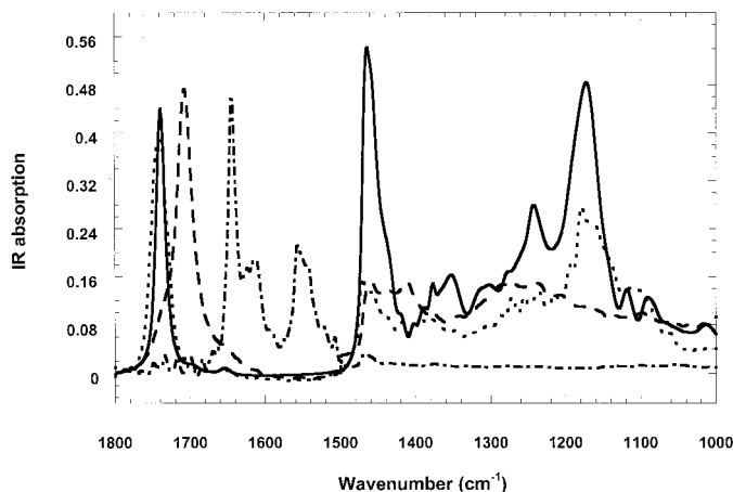
FIG. 8. Examples of IR absorption of lipid mixtures which are commonly attributed to sebum and SC are shown. (—) Triglycerides; (····) waxes; (---) free fatty acids; (-·-) ceramides. Ceramides do not have a peak in the 1800 – 1700\text{ cm}^{-1} region, and free fatty acids are the only lipid mixture that shows an absorption near 1710\text{ cm}^{-1} .
